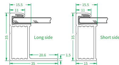
5: Frame profile
