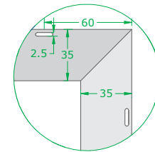
2: Drainage (x8)
