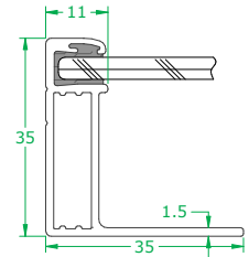
5: Frame profile
