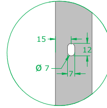
4: Mounting (x4)
